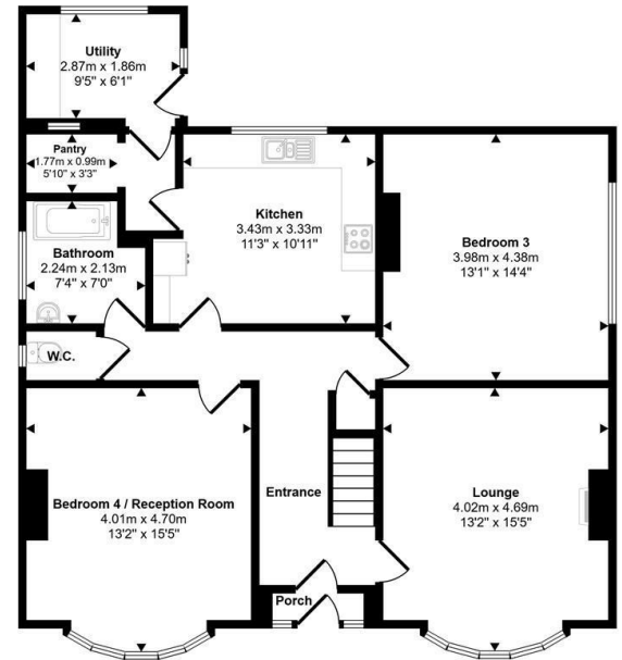
Ground Floor Approx 99 sq m / 1064 sq ft
